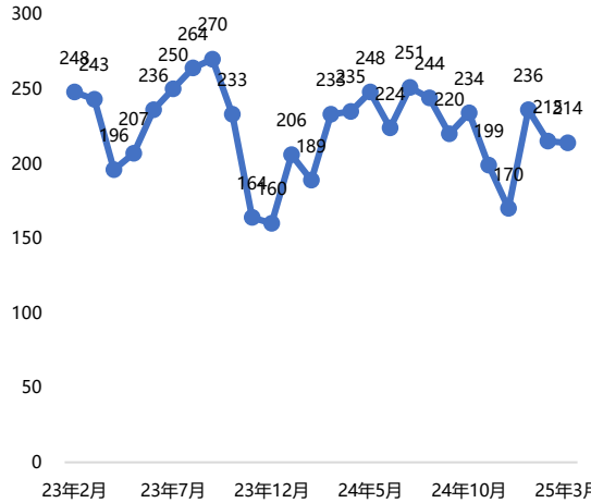
3 Resume Worded
