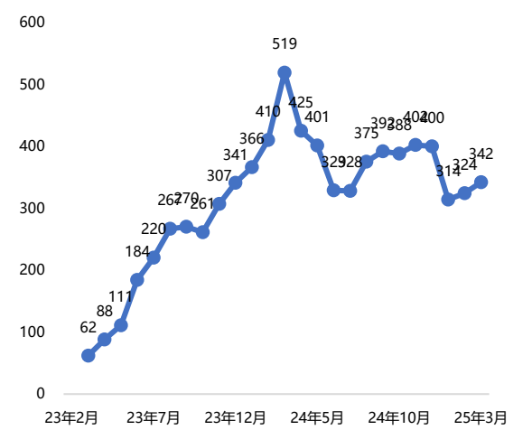
20 SnapEdit
