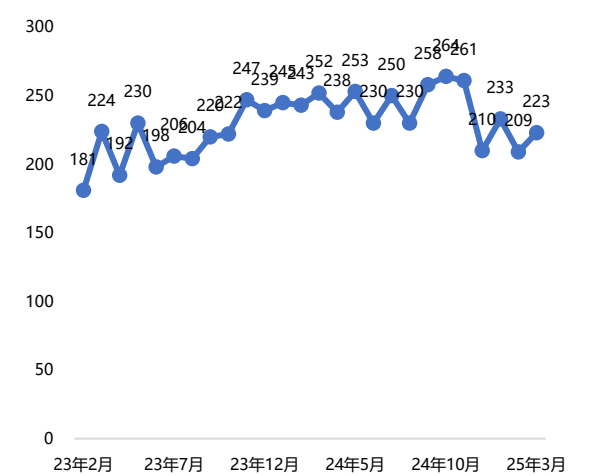
3 Whimsical
